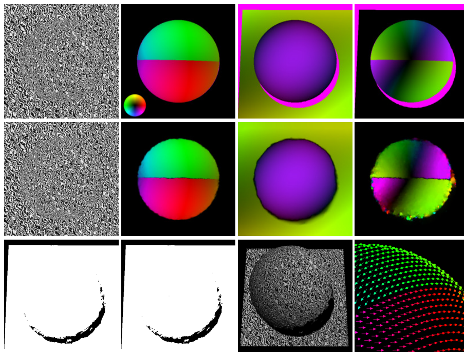
Fig. 2. Results for the general sphere sequence (image size 512 \times 512 ). Top Row: (a) Left frame at first time step. (b) + (c) + (d) Ground truth of left optical flow, first stereo flow and flow change. Colour encodes the direction, brightness the magnitude (see colour circle). Occlusions are coloured pink. Middle Row: (e) Left frame at second time step. (f) + (g) + (h) Estimated left optical flow, first stereo flow and flow change. Bottom Row: (i) + (j) Estimated occlusion scores o_{1r} and o_{2r} . (k) Estimated scene reconstruction. (l) Estimated scene flow. Runtime: \sim 420 seconds. Parameters: \alpha_1 = 1.5 , \alpha_2 = 2 , \alpha_3 = 0.8 , \beta_1 = \beta_2 = 0.03 , \gamma = 0.1 , \mu = 1 .
