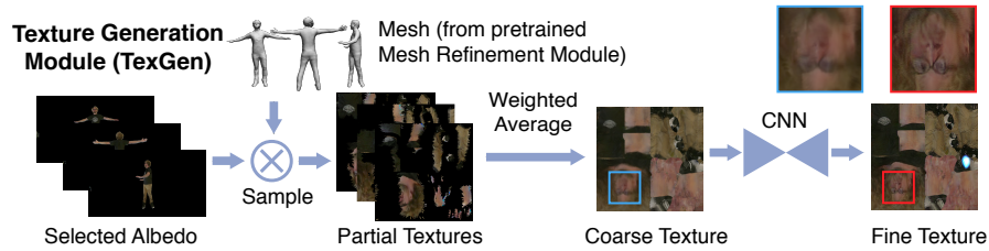
Fig. 4. Texture Generation Module (TexGen). TexGen selects K albedo images and converts them into partial textures. A coarse full texture is constructed by averaging the partial textures with weights. The texture is then refined by a CNN optimized from scratch for each video. The supervision comes from rasterizing the texture to the image space and comparing it with the input albedo images.
