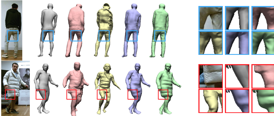
Fig. 9. Comparing mesh with coarse mesh (grey), DeepHuman [58] (red), HMD [60] (yellow), Tex2Shape [4]. Our method (green) outperforms them in shape and details: DeepHuman is coarse in head and hands. HMD has artifacts in head and body regions. Tex2Shape does not obtain realistic wrinkles.
